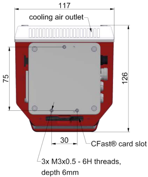
Rear View
